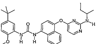
1-[4-(2-sec-Butylamino-pyrimidin-4-yloxy)-naphthalen-1-yl]-3-(5-tert-butyl-2-methoxy-phenyl)-urea;
